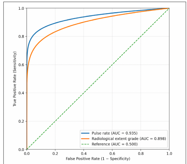
Figure 1. Receiver operating characteristic (ROC) curves illustrating the discriminative performance of pulse rate and radiological extent grade for predicting in-hospital mortality in patients with Fournier's gangrene.
