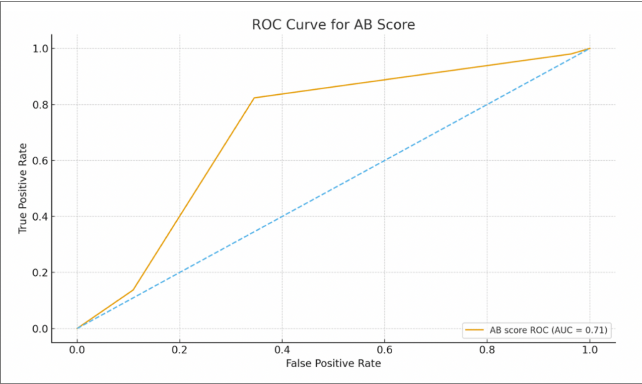
Figure 1. Receiver operating characteristic (ROC) curve of the Antoine B  cl  re (AB) score for predicting the need for operative intervention in adhesive small bowel obstruction. ROC curve illustrating the discriminative performance of the AB score for predicting operative intervention in patients with adhesive small bowel obstruction. The area under the curve (AUC) was 0.71, indicating acceptable discriminative ability. Using a cutoff value of AB ≥2, the score demonstrated a sensitivity of 82% and a specificity of 66% for identifying patients who ultimately required surgery.
